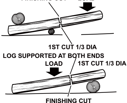
LOG SUPPORTED AT ONE END Fig. 17 FINISHING CUT LOAD
